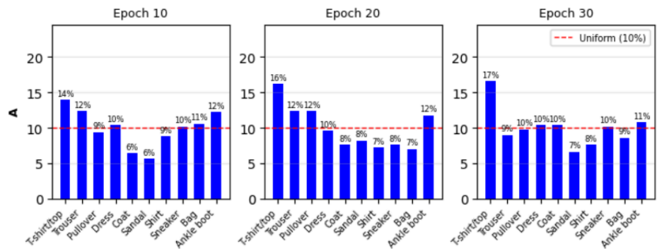
Figure 9. Classifier-based assessment of 500 generated images at epochs 10, 20, 30 of GAN training using the classifier from task 1. figure row A, the bars show the percentage of generated images assigned to each Fashion MNIST class; the red dashed line marks the 10% uniform expectation and deviation indicates partial mode collapse.
